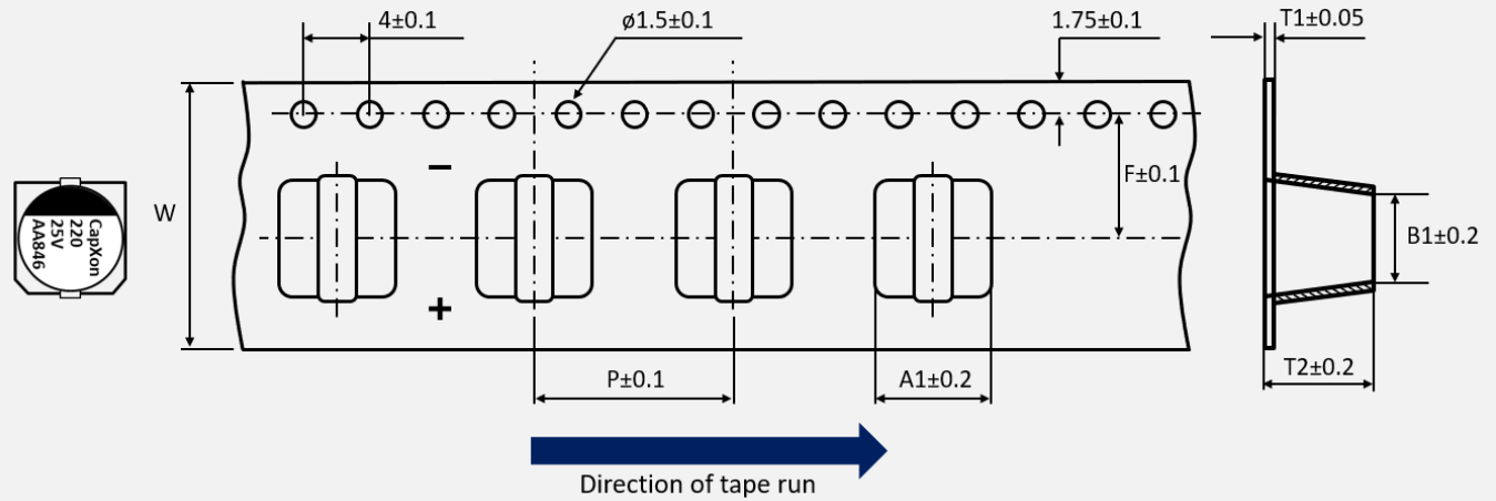
SMD taping • \phi D 5mm to 10mm
